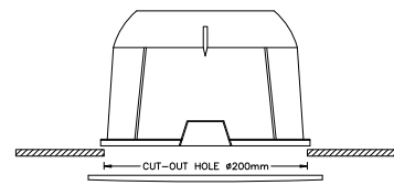
CUT-OUT DETAILS
